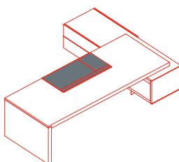
Left desk arranged for electrification, with black leather lifttable desk pad and side container 1AS4832: L 272 D 200 H 75
