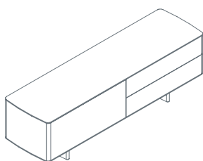
Storage lockable unit, 1 left filing drawer and 2 right drawers 1SH5030: L 190 D 53 H 59
